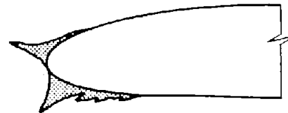
(c) Double-peak mushroom-type glaze ice. Datum air temperature, 25^{\circ} to 30^{\circ} F; moderate to high rate of water catch.
