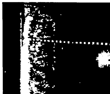
(b) Airspeed, 260 miles per hour; datum air temperature, 30° F; liquid-water content, 0.52 gram per cubic meter; angle of attack, 8°; icing time, 33 minutes; initial drag coefficient, 0.0128; drag coefficient with ice, 0.0153.
