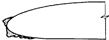
(b) Glaze ice. Datum air temperature, 25^{\circ} F; low rate of water catch.
