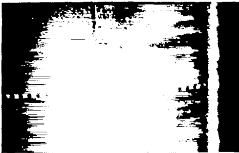
(b) Icing time, 8 minutes. Drag coefficient, 0.0204. Leading-edge upper surface.
