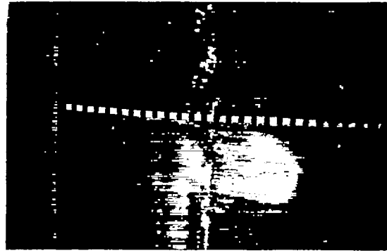
(b) Icing time, 9\frac{1}{2} minutes. Drag coefficient, 0.00973. Lower surface, after ice removal.
