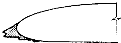
(a) Rime ice. Datum air temperature, 0^{\circ} F.
